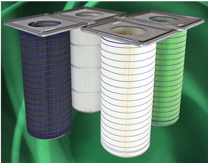
Nano fiber media filters with a rating of MERV 15 per ASHRAE 52.2:2007 are recommended in order to meet thermal spray emission regulations.
