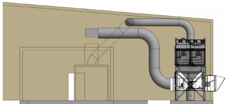
Schematic view of plasma spray booth with 24-cartridge dust collector and heated makeup air system.
