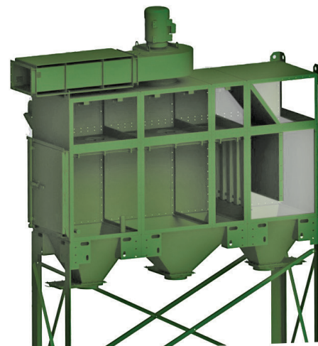
Drop-out module enhances cleaning efficiency by capturing a large quantity of dust before it reaches the primary dust collector.
