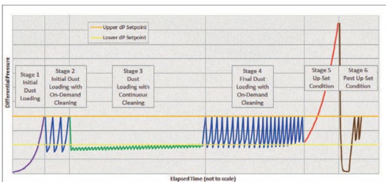
ANSI/ASHRAE Standard 199 Figure 4.1 – Schematic showing sequence of test stages.
