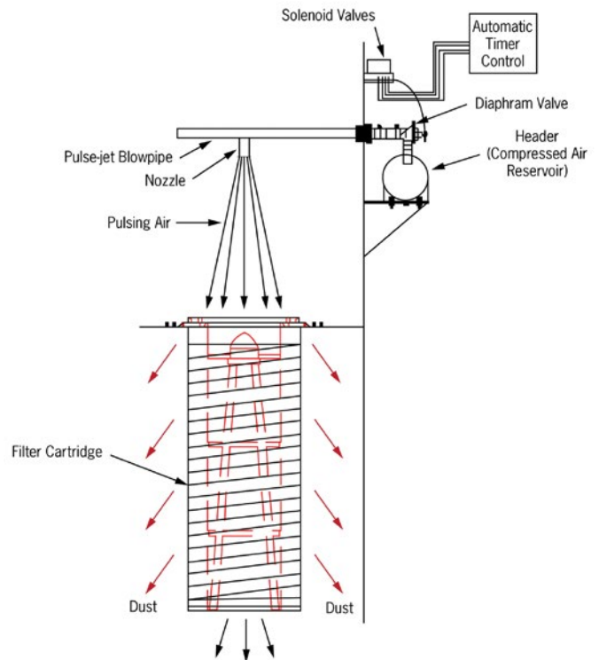
Schematic of typical pulse cleaning system used in an industrial dust collector.
