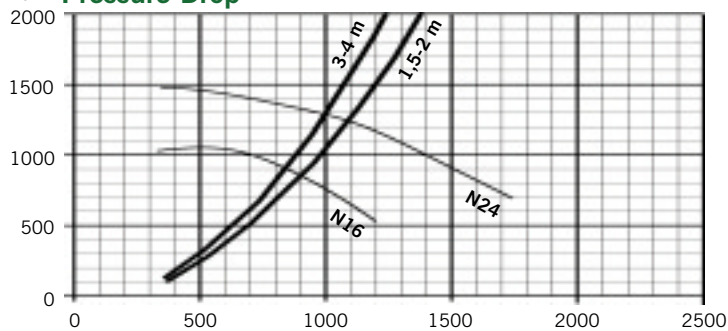
The graph shows variations of pressure drop with air flow in the various Farr Arm™ models when installed in the normal working orientation.
